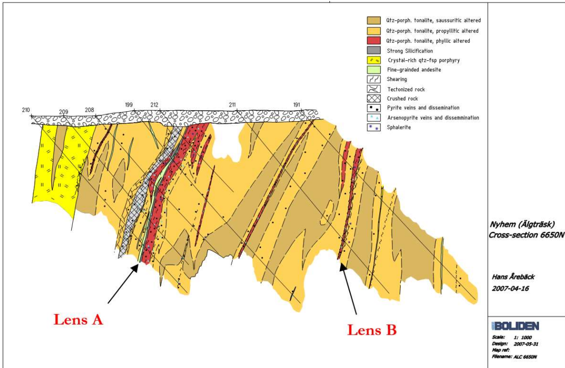
Figure 6. Cross section perpendicular to strike illustrating the steeply dipping vein type mineralisations in Nyhem area.
