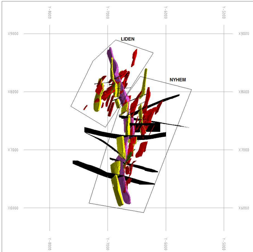
Figure 7. Älgräsk Liden and Nyhem 3D geological model of the mineralized (red) zones with greenstone (green), QFD dykes (yellow), fault structures (black) and crushed zone (purple).
